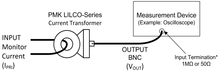
Figure 2 - Basic Connection to the Circuit Under Test
