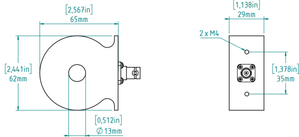
Figure 3 - PMK LILCO®-Series 13 Mechanical Dimensions
