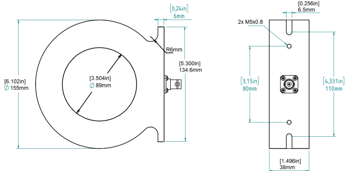
Figure 5 - PMK LILCO®-Series 89 Mechanical Dimensions
