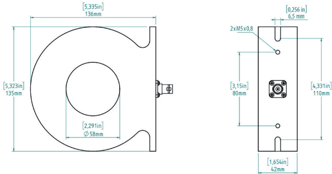
Figure 4 - PMK LILCO®-Series 58 Mechanical Dimensions
