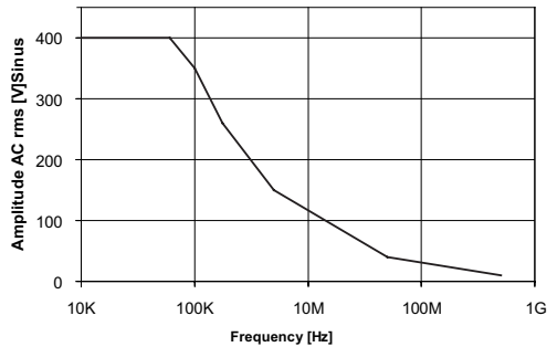
Typical voltage derating PKT512A-RO Measurement Category I
