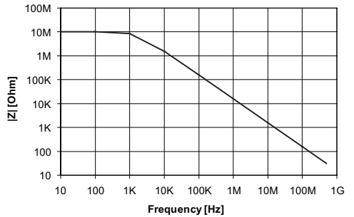
Typical input impedance PKT512A-RO
